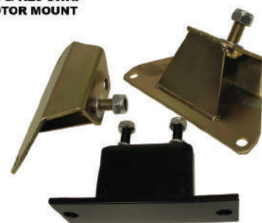
MM-015 1996 - 2004 FORD MUSTANG GT/LX/COBRA 4.6L HEAVY DUTY MOTOR MOUNT
